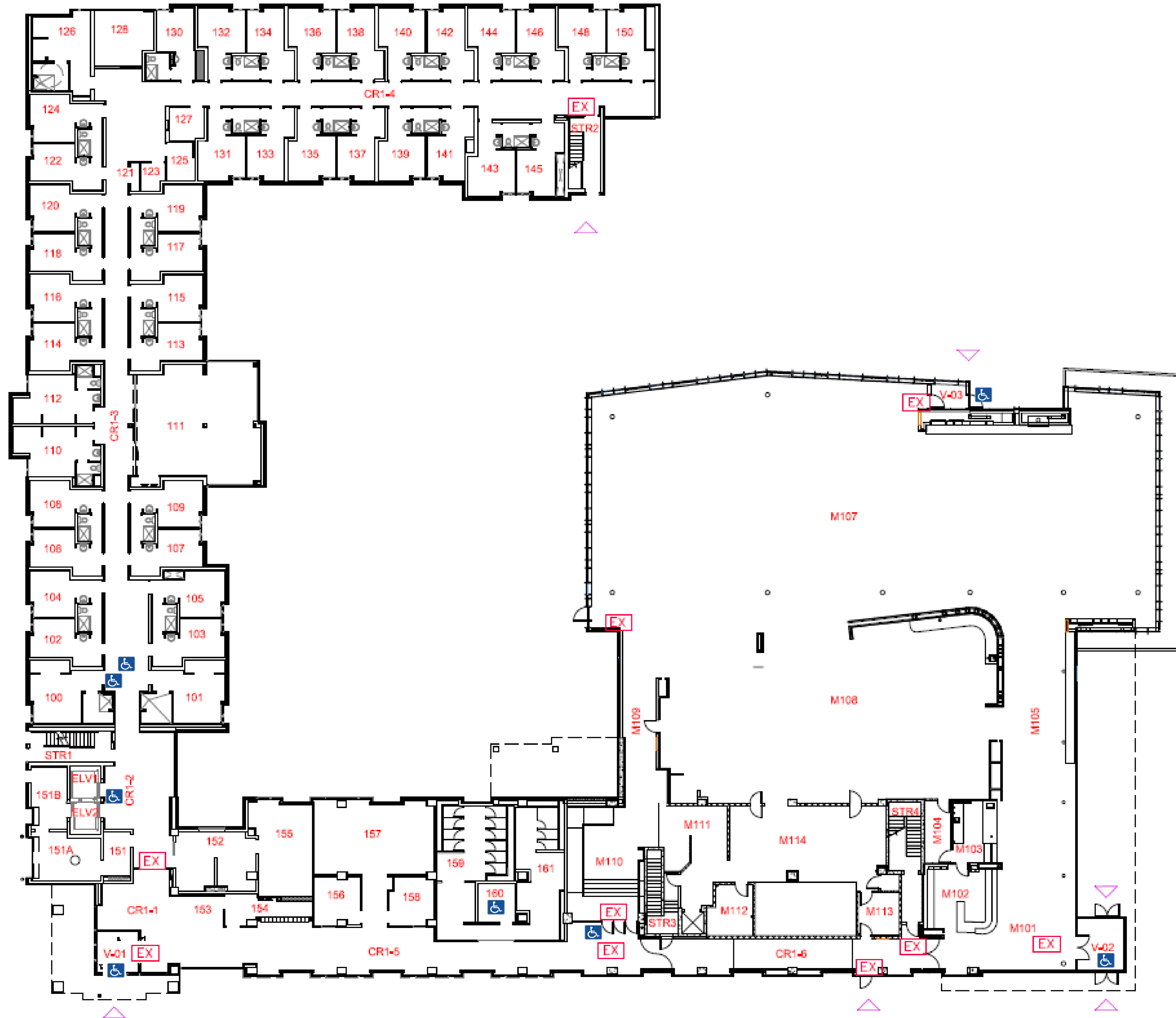
CLARE HALL - 2nd - 4th FLOOR
